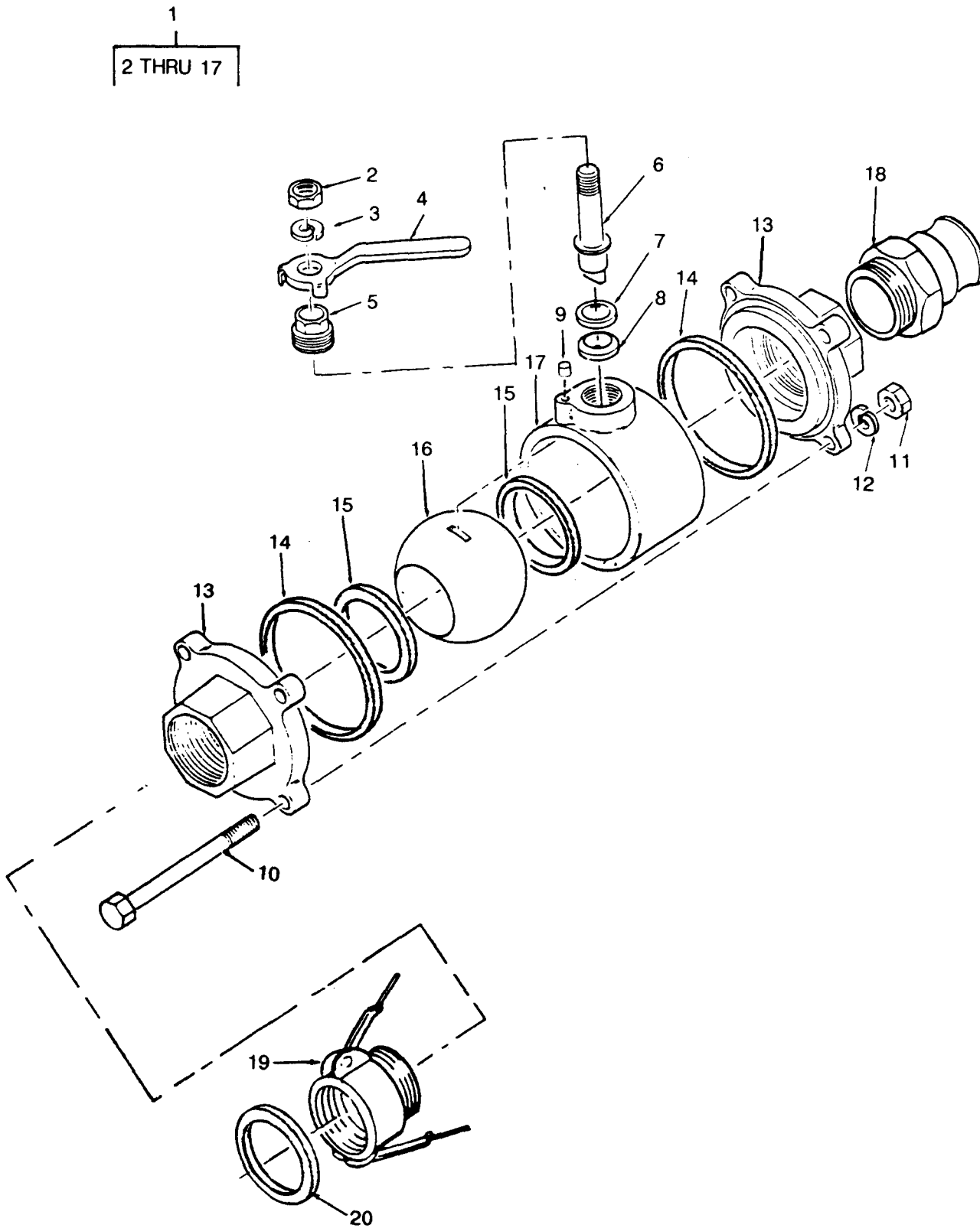
Figure 1. Ball Valve, Quick Acting
